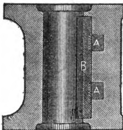
ELEVATION (TAPPET).
