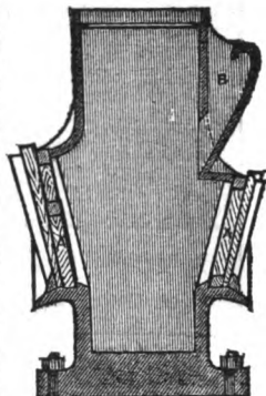
DOUBLE-DISCHARGE MORTAR. (End View.)
