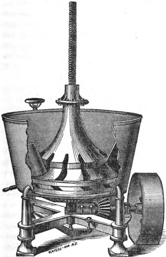
EXCELSIOR GRINDER AND AMALGAMATOR.
