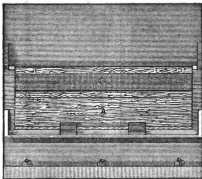
DOUBLE-DISCHARGE MORTAR. (Side View.)
